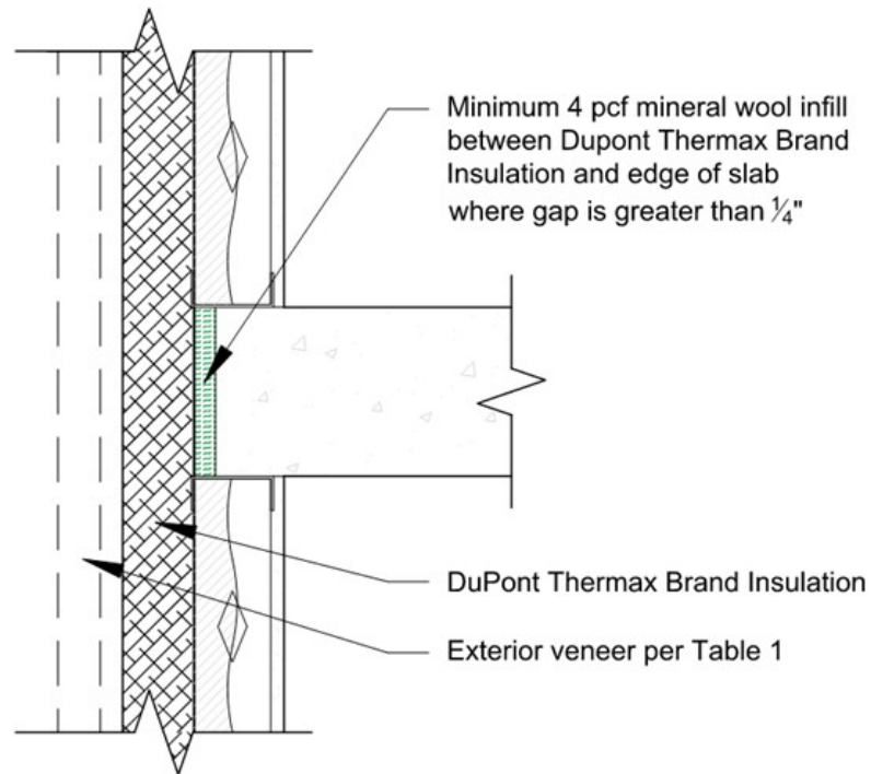
Figure 1. In-fill frame construction floor lining condition
