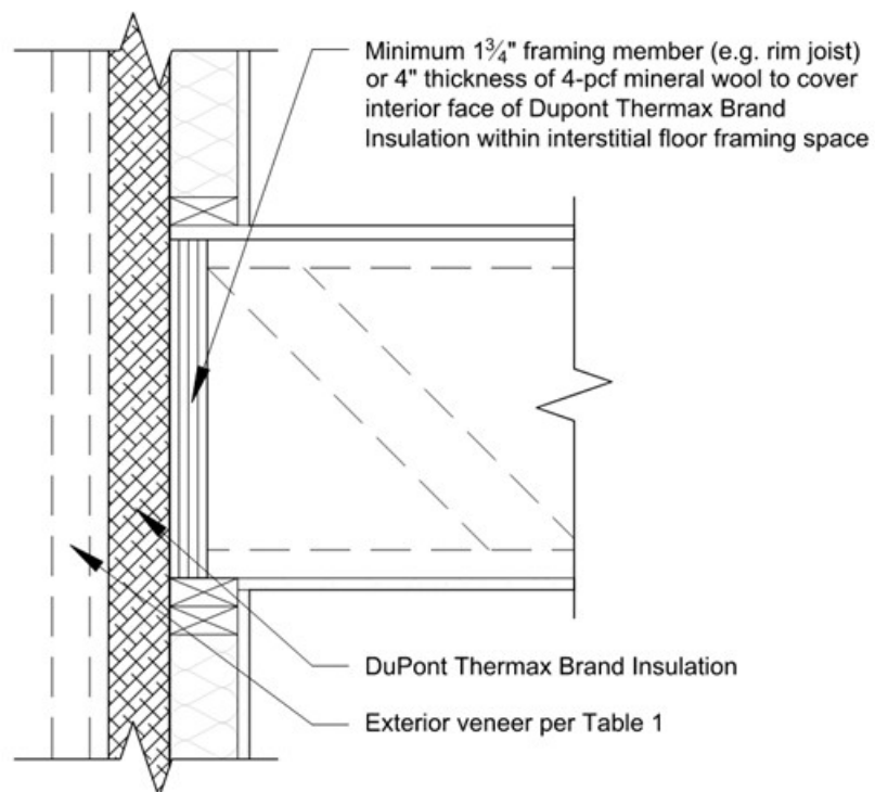
Figure 2. Platform frame construction floor line condition
