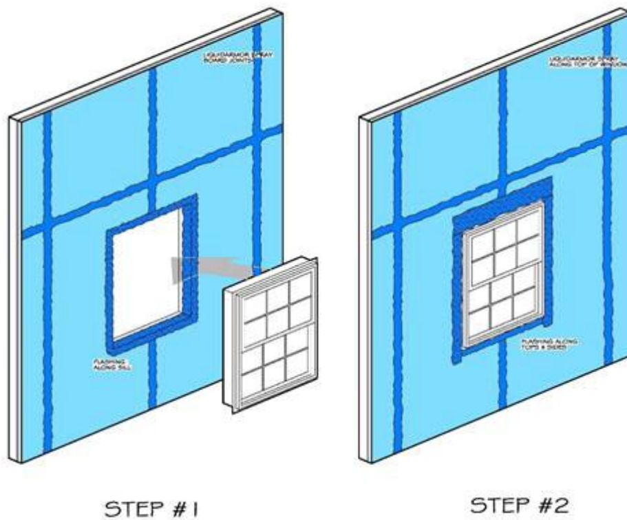
FIGURE 21—TYPICAL WINDOW FLASHING DETAIL
