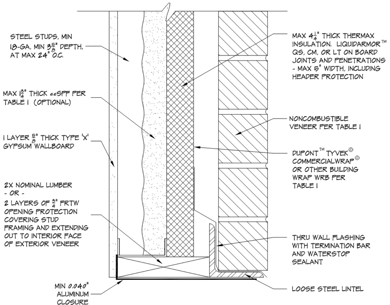
Figure 13 – Exterior wall construction – Thermax and ccSPF spray foam – Table 5 Opening Protection Item 31c
