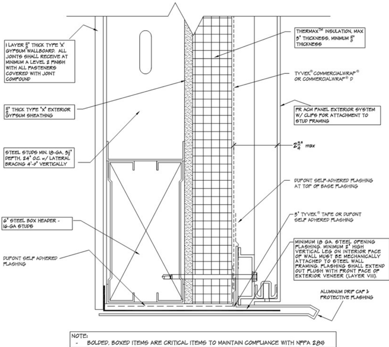
Figure 17 – Use of water-resistive barrier over Thermax insulation – Table 3
