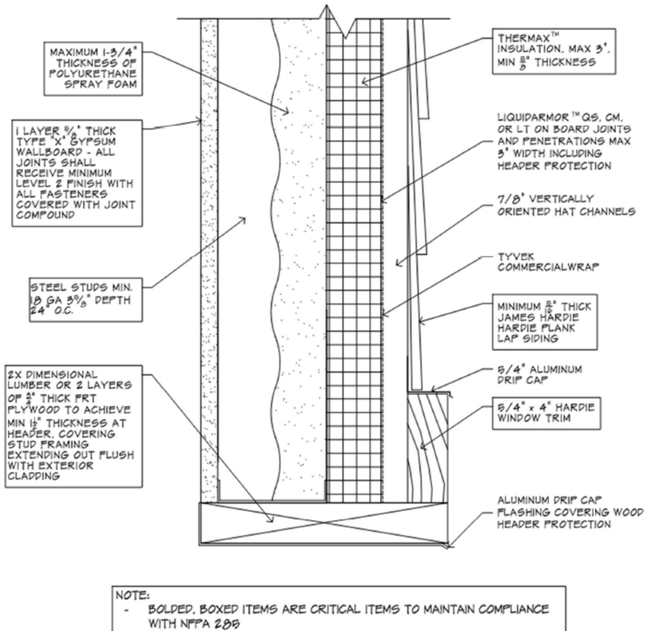
Figure 10 – Wall opening perimeter protection (header shown) – one layer of nominal 2x lumber of two layers of 3/4-in.-thick FRT plywood covering full depth of wall system – Table 4, Item 33c
