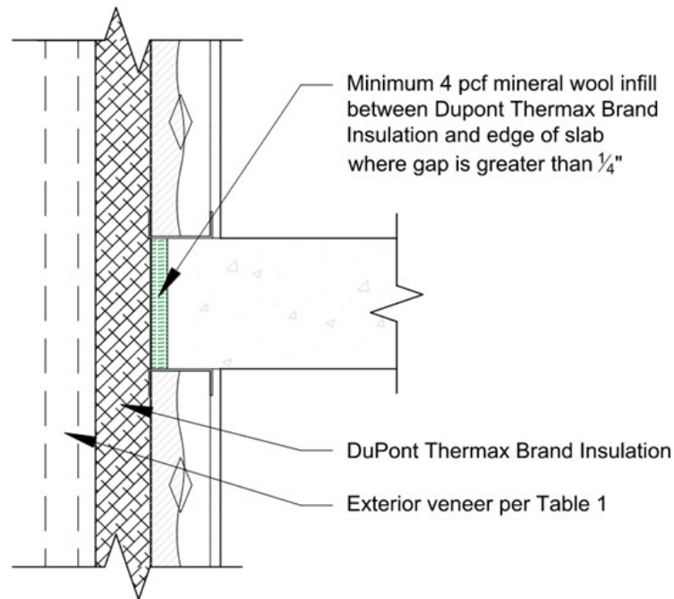
Figure 1 – In-fill Frame Construction Floor Line Condition
