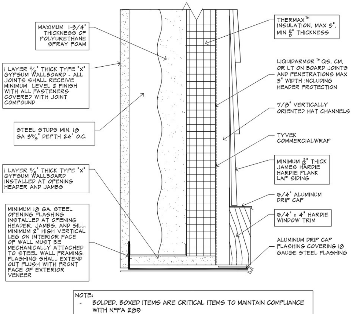
Figure 8 – Wall opening protection (header shown) – 5/8-in.-thick Type X gypsum wallboard covering stud framing and exposed edge of Thermax insulation with 18-ga. steel flashing at header, jambs and sill – Table 4, Item 33a
