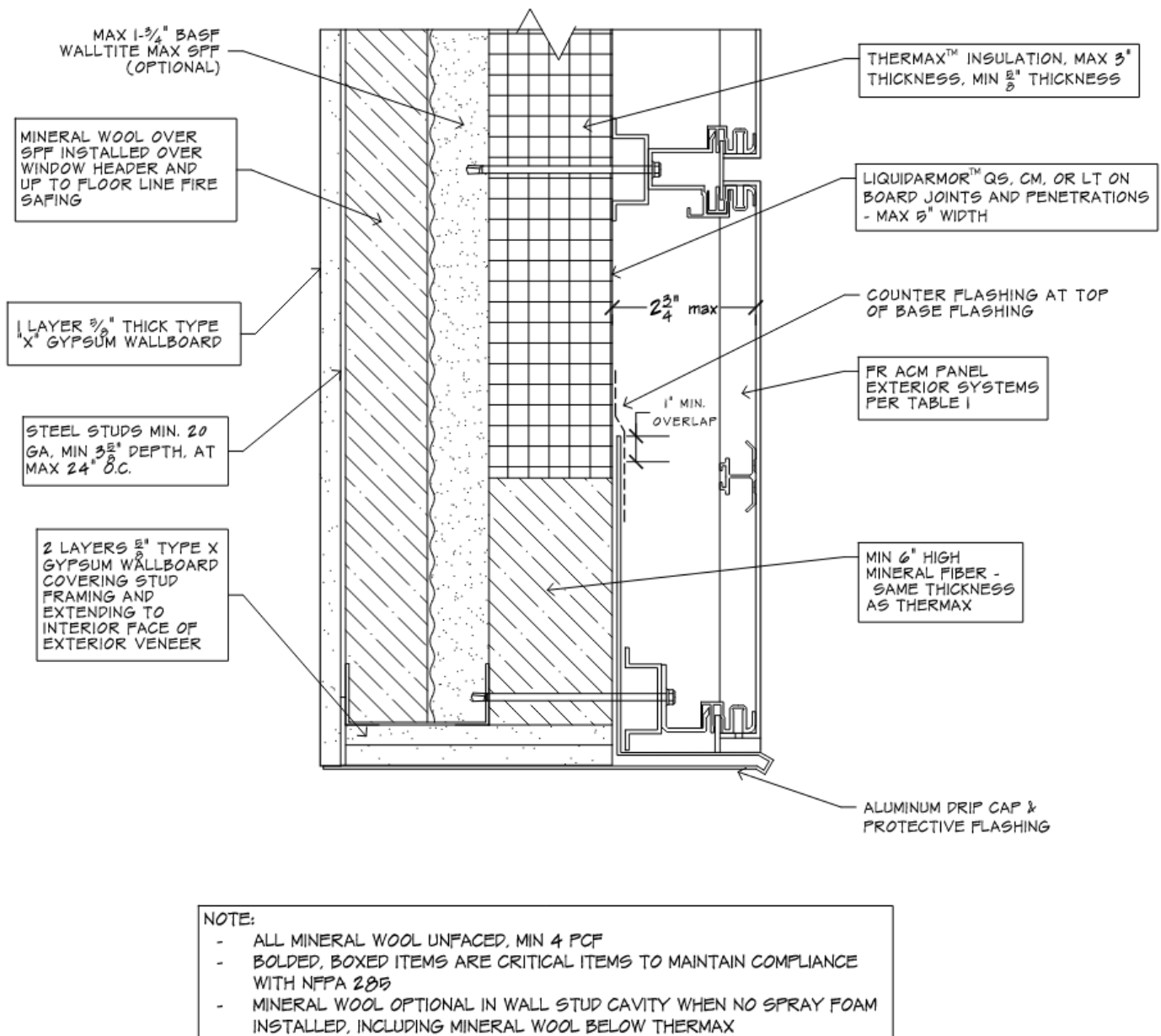
Figure 6 – Wall opening perimeter protection (header shown) – 5/8-in.-thick Type X gypsum wallboard at header, jambs and sill – Table 3, Item 23b
