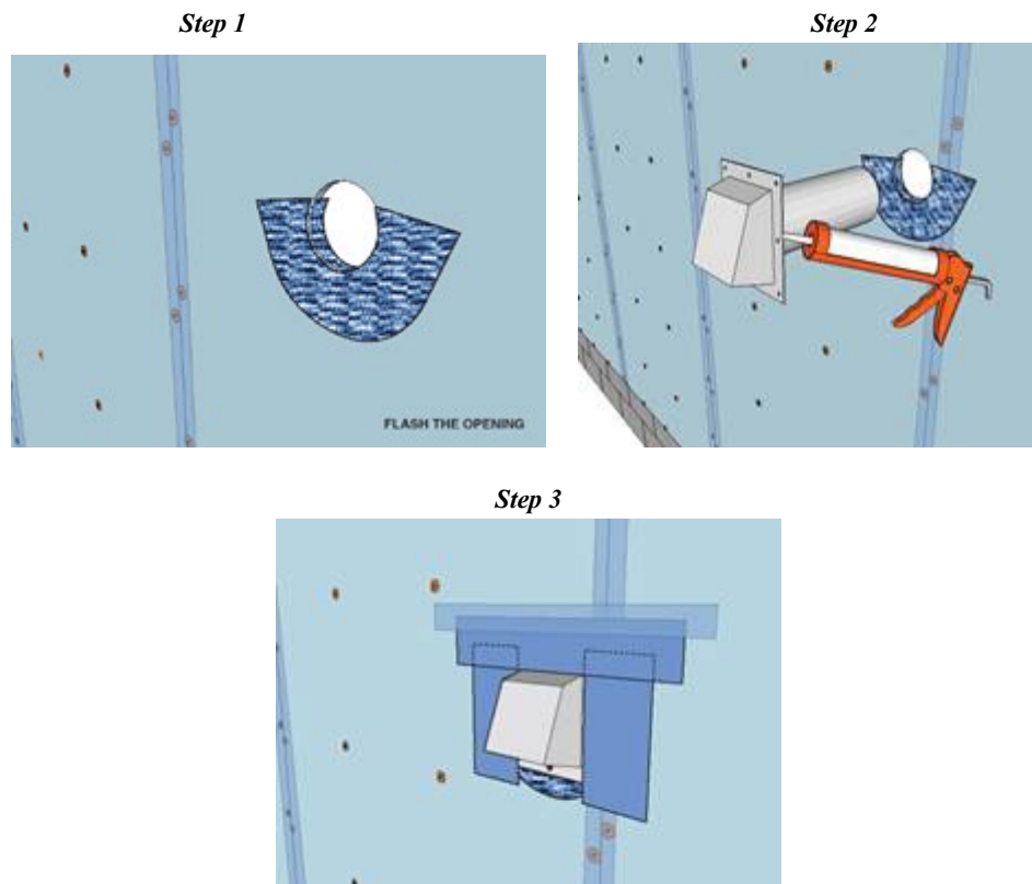
FIGURE 19—TYPICAL PENETRATION FLASHING DETAIL—FLANGED
