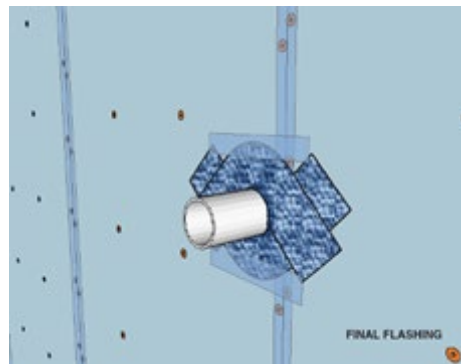
FIGURE 20—TYPICAL FLASHING DETAIL—UNFLANGED
