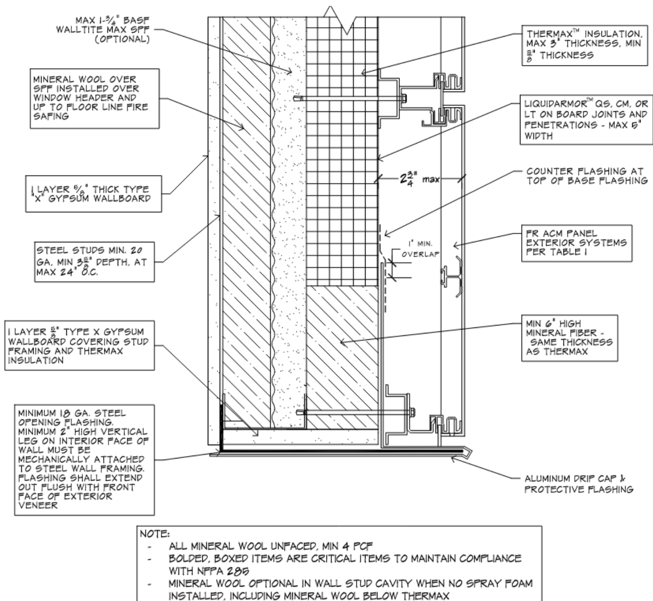
Figure 5 – Wall opening protection (header shown) – 5/8-in.-thick Type X gypsum wallboard at header and jambs, 18-ga. steel flashing at header, jambs and sill – Table 3, Item 23a
