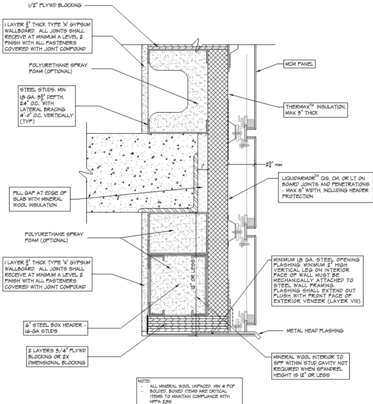
Figure 15 – Required opening head protection for infill wall construction with ACM Façade – Table 3
