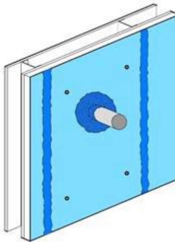
FIGURE 23—TYPICAL FLASHING DETAIL—UNFLANGED
