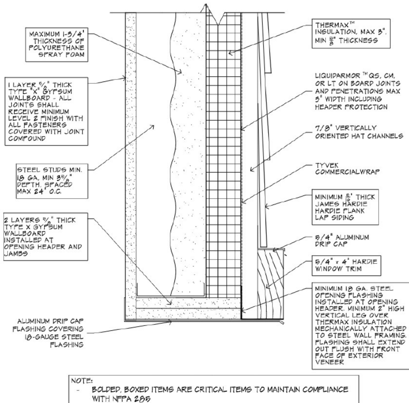
Figure 9 – Wall opening perimeter protection (header shown) – two layers of 5/8-in.-thick Type X gypsum wallboard covering steel framing and exposed edge of Thermax insulation with 18-ga. steel flashing continuing outboard to exterior cladding – Table 4, Item 33b.
