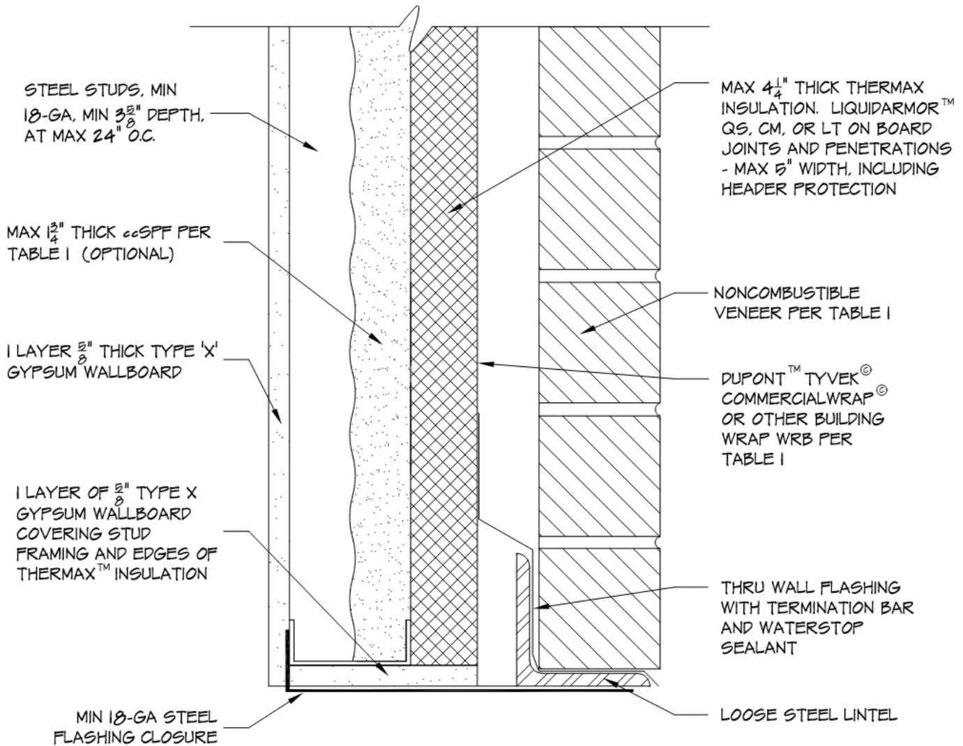
Figure 11 – Exterior wall construction – Thermax and ccSPF spray foam – Table 5 Opening Protection Item 31a
