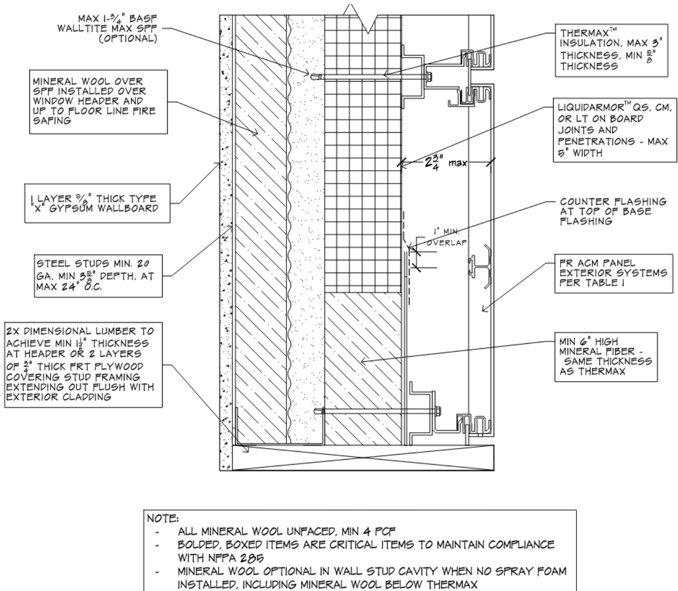
Figure 7 – Wall opening perimeter protection (header shown) – 2x dimensional lumber or double 3/4-in. FRT plywood at header, jambs and sill – Table 3, Item 23c
