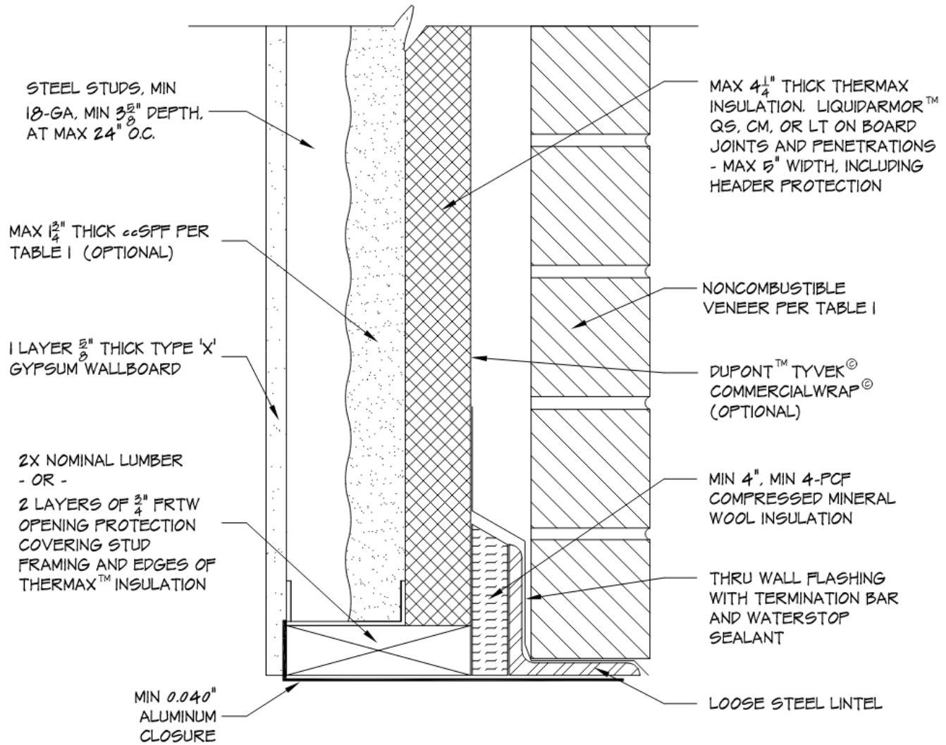
Figure 14 – Exterior wall construction – Thermax and ccSPF spray foam – Table 5 Opening Protection Item 31d
