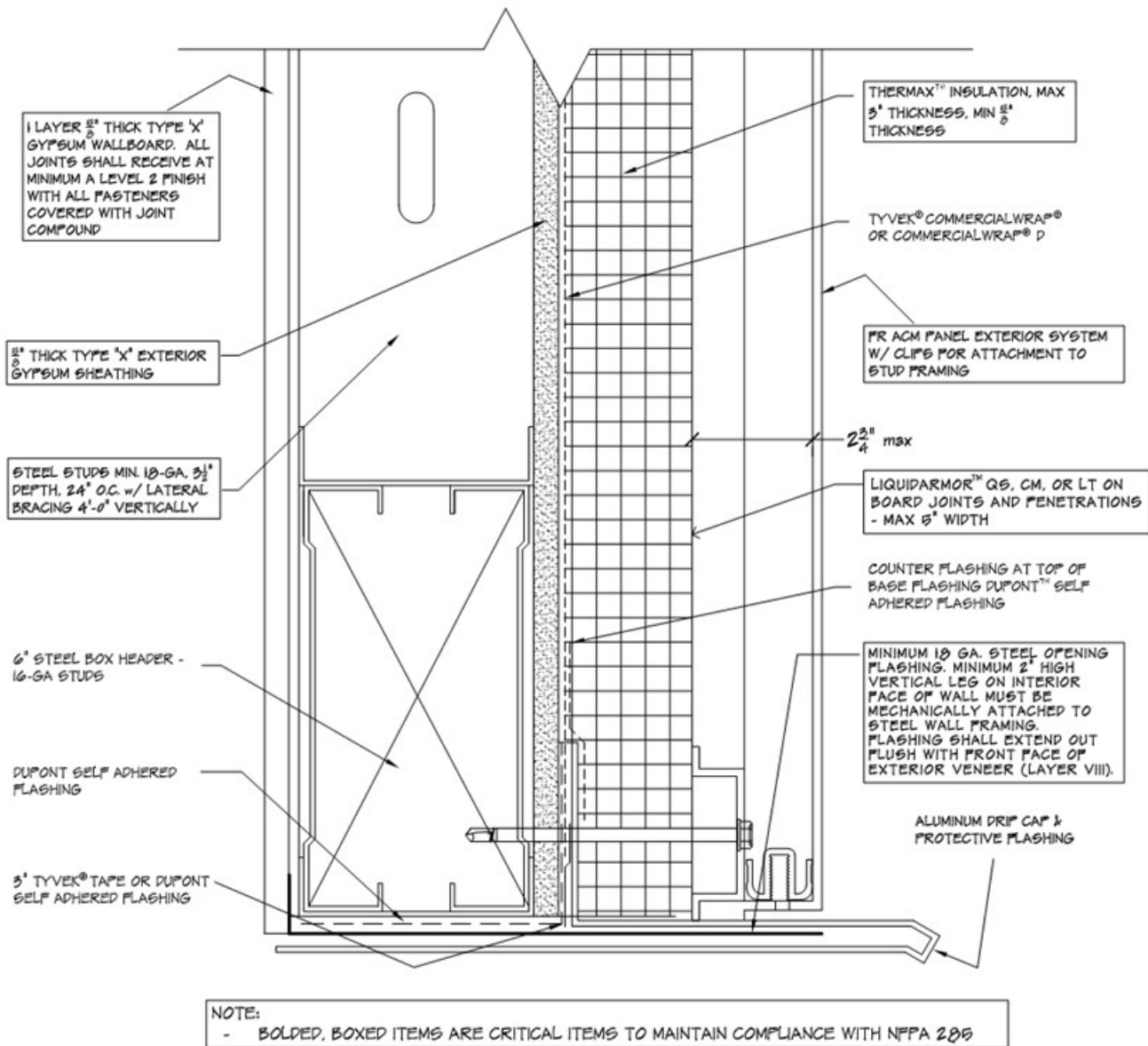
Figure 16 – Use of water-resistive barrier behind Thermax insulation – Table 3
