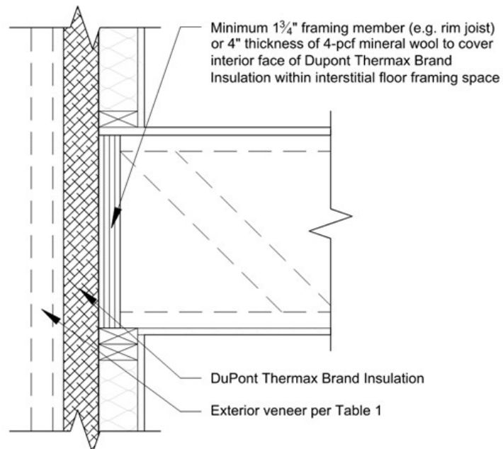
Figure 2 – Platform frame construction floor line condition
