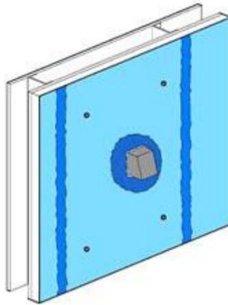
FIGURE 22—TYPICAL PENETRATION FLASHING DETAIL—FLANGED
