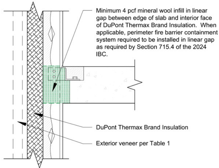
Figure 3 – Curtain wall frame construction floor line condition
