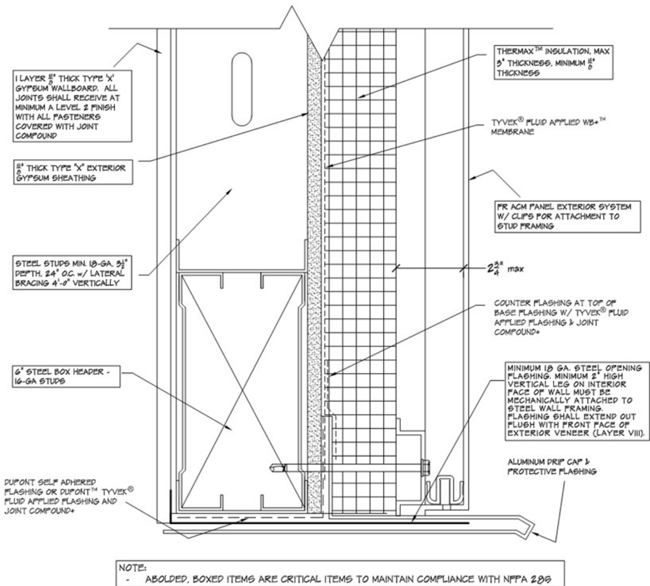
Figure 18 – Use of fluid-applied water-resistive coating behind Thermax insulation – Table 3
