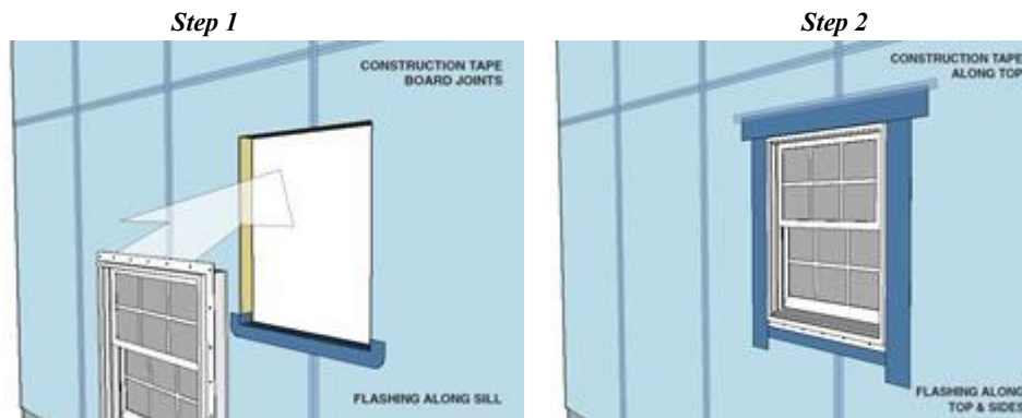
FIGURE 19—TYPICAL WINDOW FLASHING DETAIL
