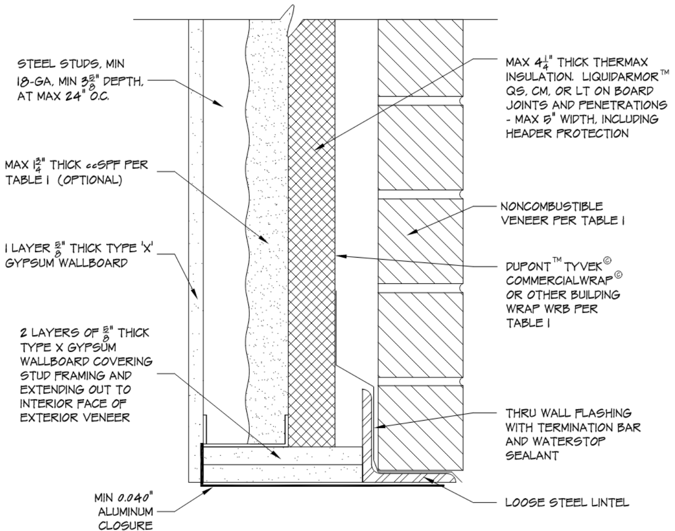
Figure 12 – Exterior wall construction – Thermax and ccSPF spray foam – Table 5 Opening Protection Item 31b
